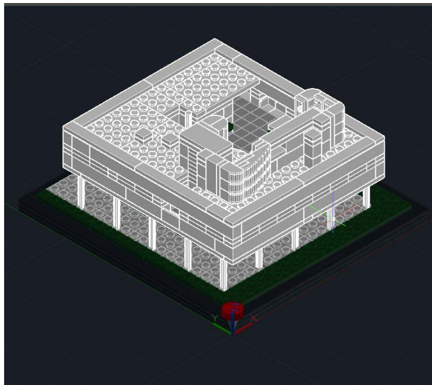
Autodesk AutoCAD 2015
