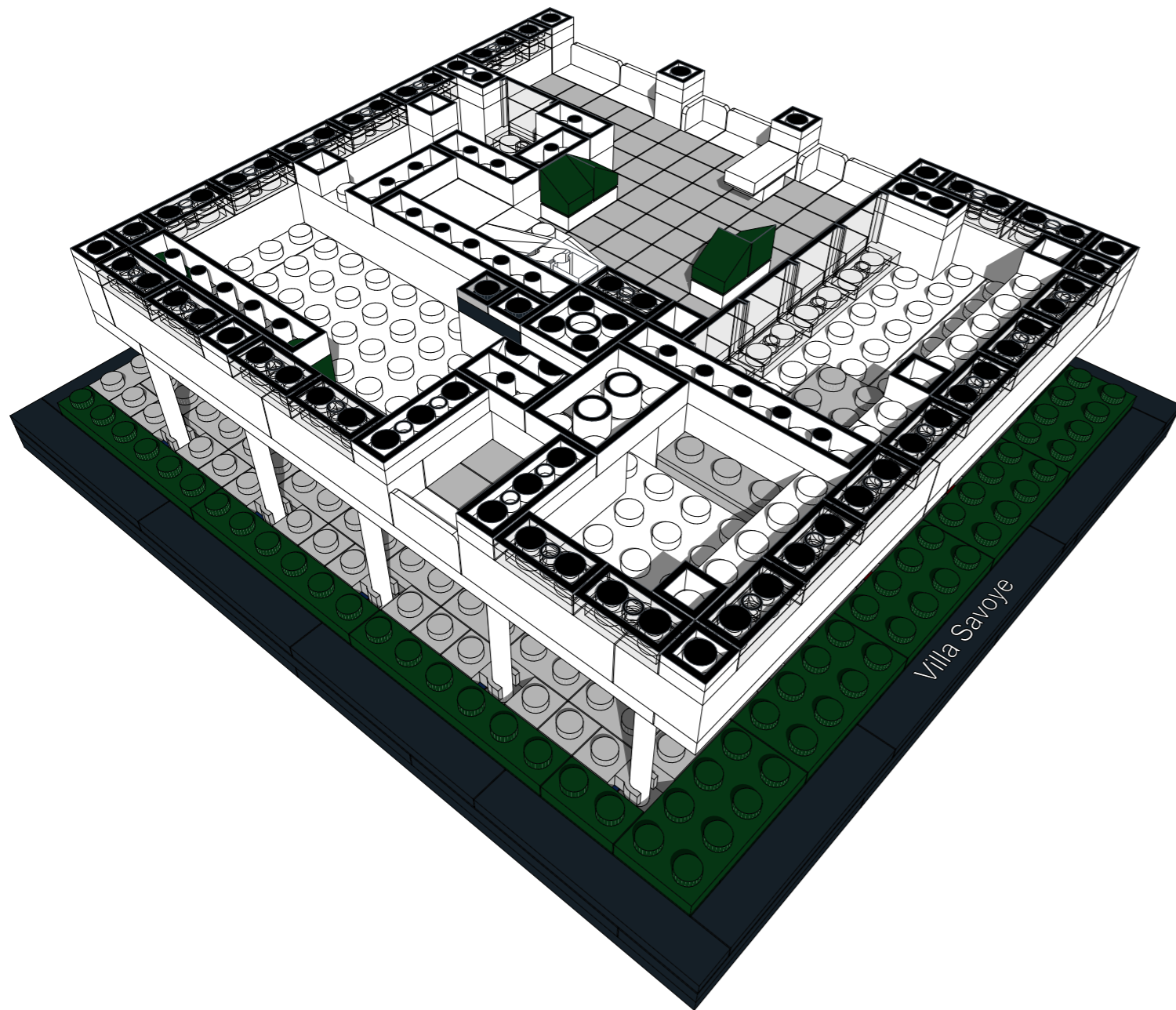
Cut View 1 - Horizontal
